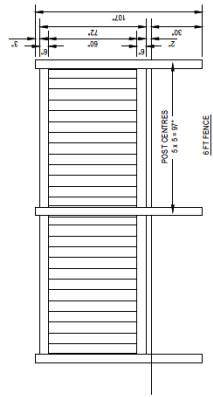
1 PRIVACY FENCE - VINYL N.T.S. NOTES: 1. FENCE SHALL BE INSTALLED IN ACCORDANCE WITH LOCAL CODES. 2. ALL MATERIALS SHALL BE APPROVED BY ARCHITECTURAL REVIEW COMMITTEE. 3. INSTALLATION TO BE COMPLETED IN ACCORDANCE WITH MANUFACTURER'S SPECIFICATIONS. 4. FINISH COLOR TO BE SPECIFIED BY ARCHITECTURAL REVIEW COMMITTEE. 5. FINISH COLOR TO BE APPROVED BY ARCHITECTURAL REVIEW COMMITTEE. 6. FINISH COLOR TO BE APPROVED BY ARCHITECTURAL REVIEW COMMITTEE. 7. ARCHITECTURAL FINISHES TO BE APPROVED BY ARCHITECTURAL REVIEW COMMITTEE.
