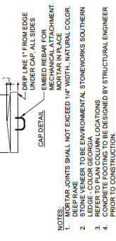
5 FENCE COLUMN N.T.S. NOTES: 1. MORTAR JOINTS SHALL NOT EXCEED 1/4\"/>
